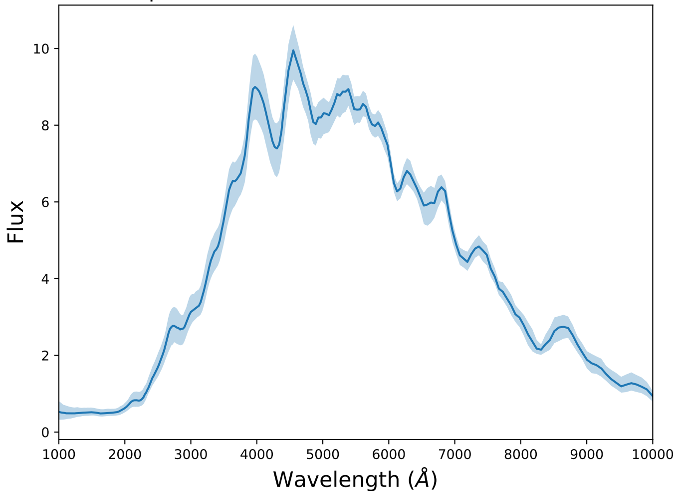
Spectrum 7 for transient SNIax at z=0.64
